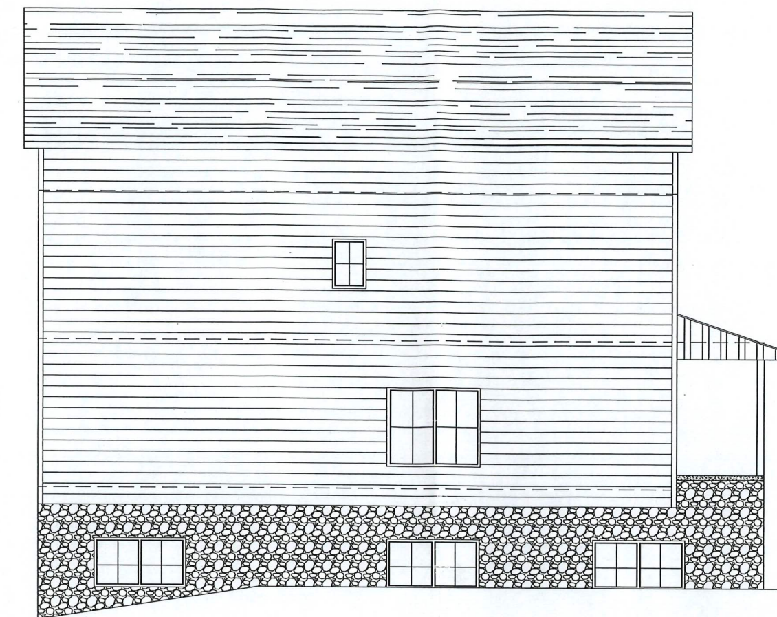
LEFT ELEVATION
