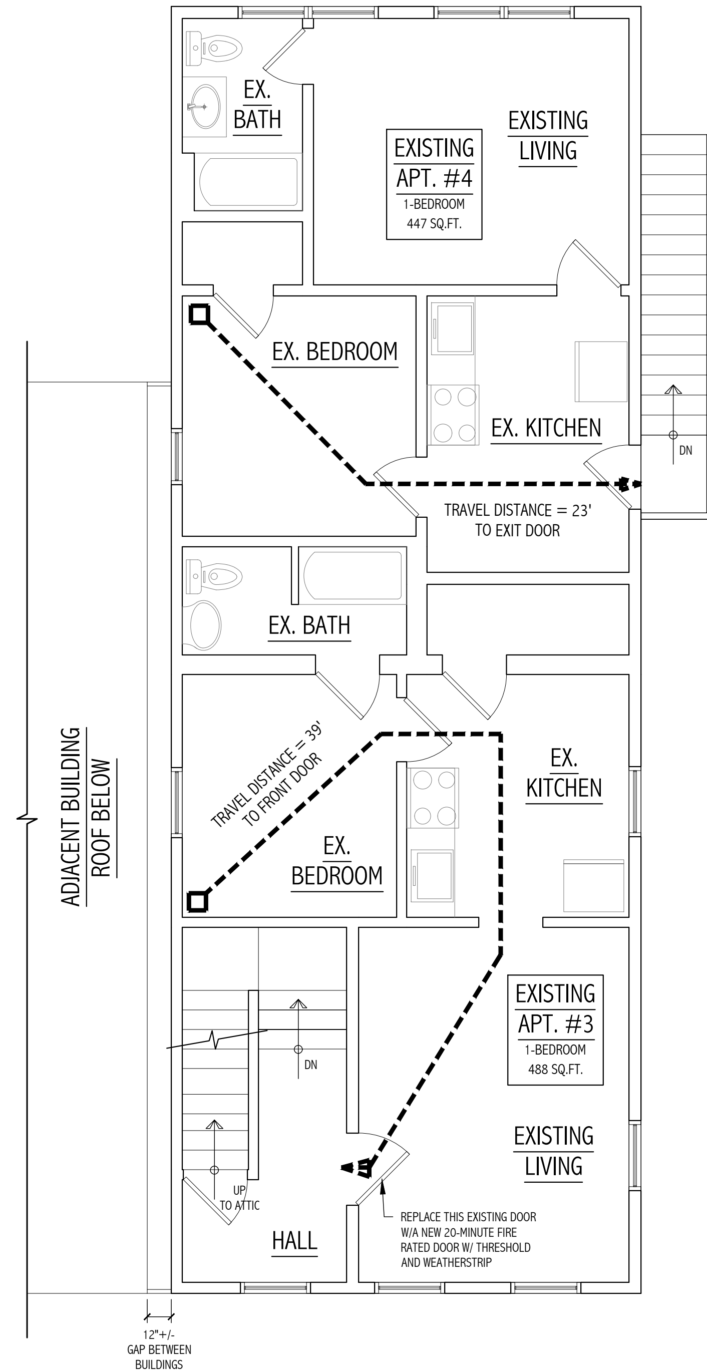
1 SECOND FLOOR PLAN A-1 1/4\"/>
