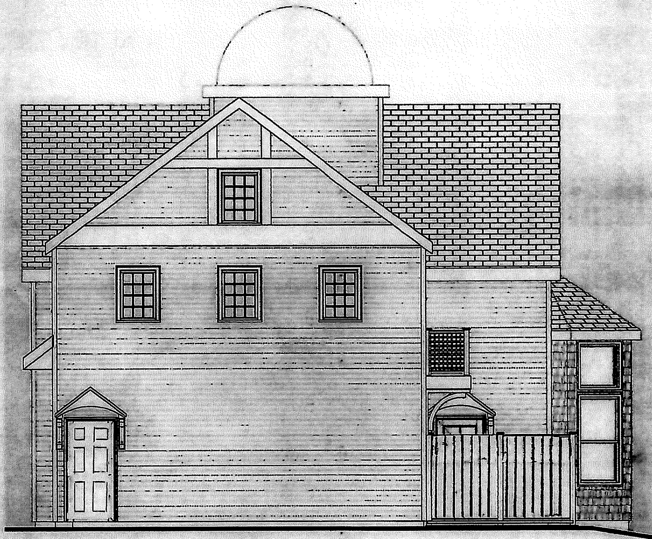
5 ARCH. - WEST ELEVATION (SIDE) SD 1/4" = 1'-0"
