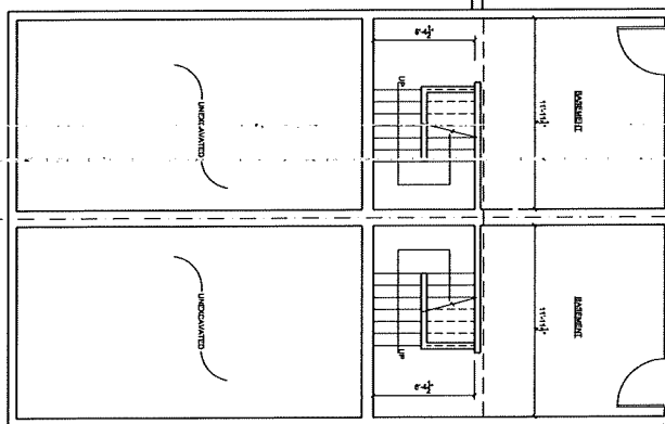
4 BASEMENT PLAN SCALE: 1/8" = 1'-0"
