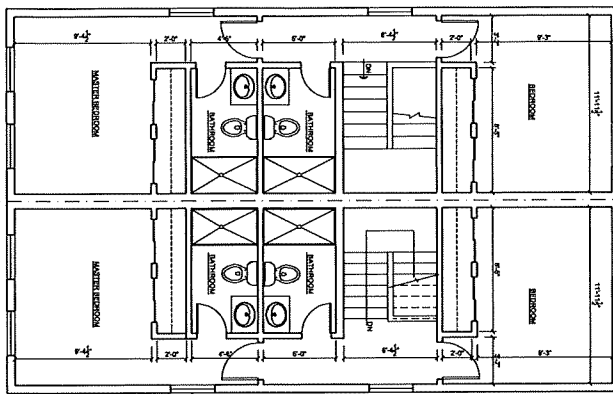
1 THIRD FLOOR PLAN SCALE: 1/8" = 1'-0"
