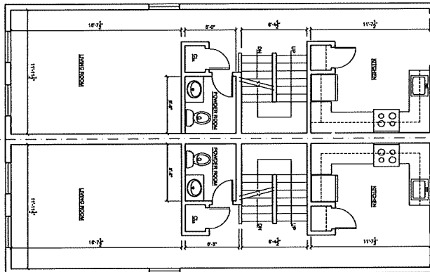
2 SECOND FLOOR PLAN SCALE: 1/8" = 1'-0"
