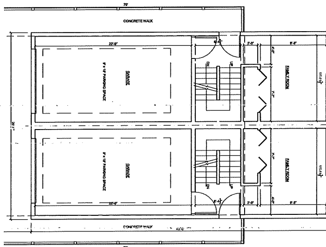
3 FIRST FLOOR PLAN SCALE: 1/8" = 1'-0"
