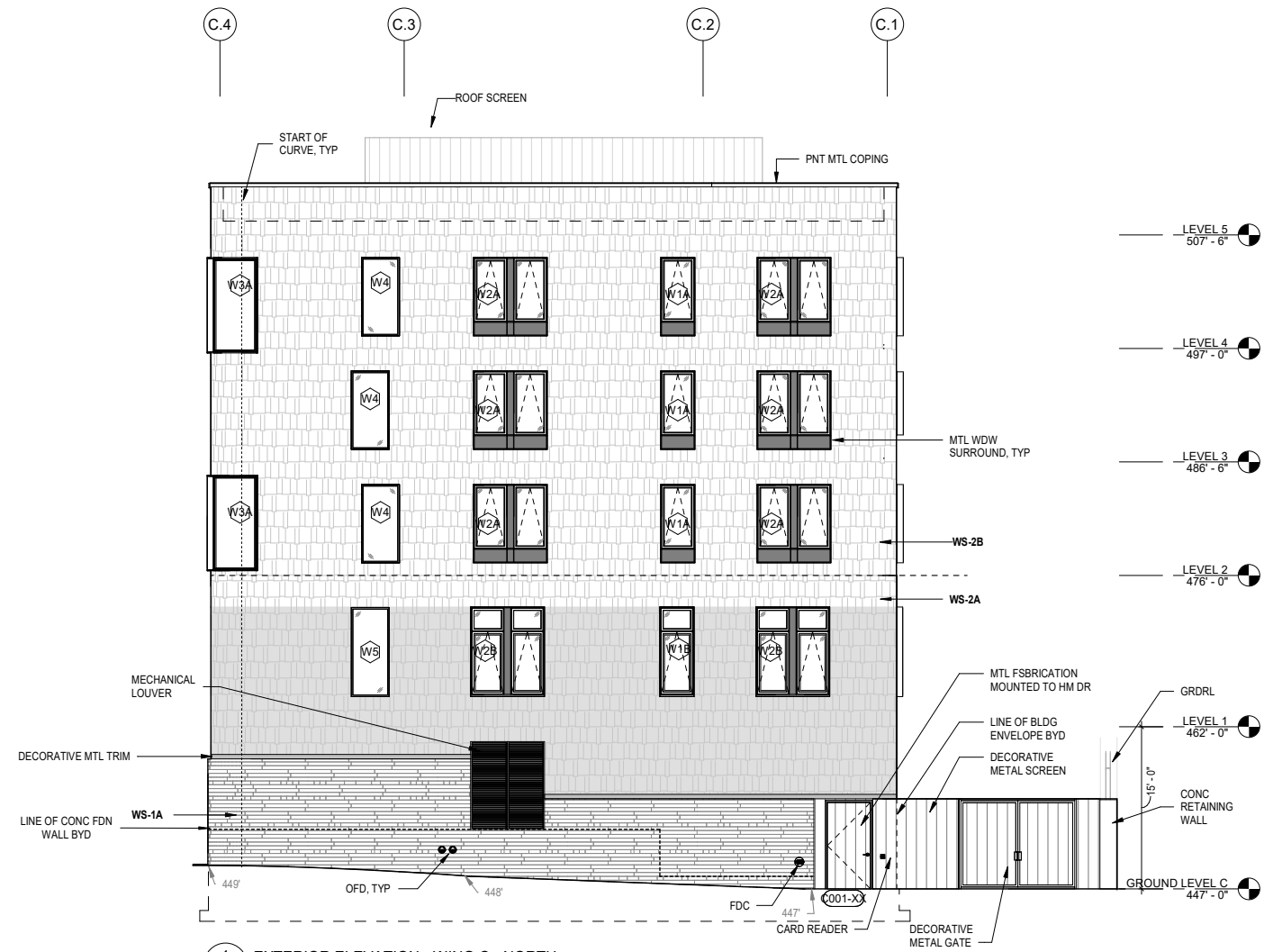
1 EXTERIOR ELEVATION - WING C - NORTH A312 1/16" = 1'-0"
