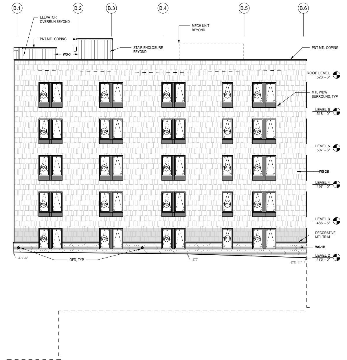
2 EXTERIOR ELEVATION - WING B - SOUTH A311 1/16" = 1'-0"
