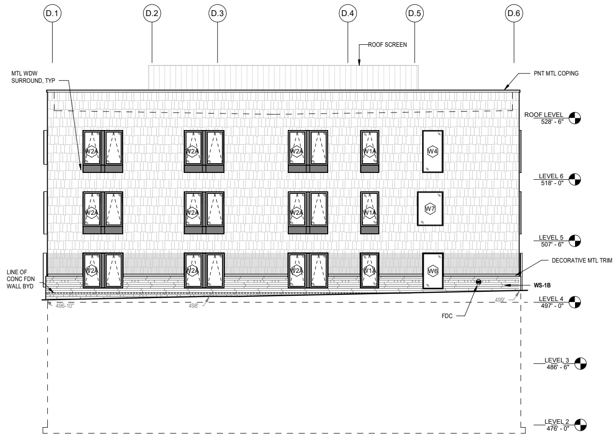
1 EXTERIOR ELEVATION - WING D - SOUTH A313 1/16" = 1'-0"
