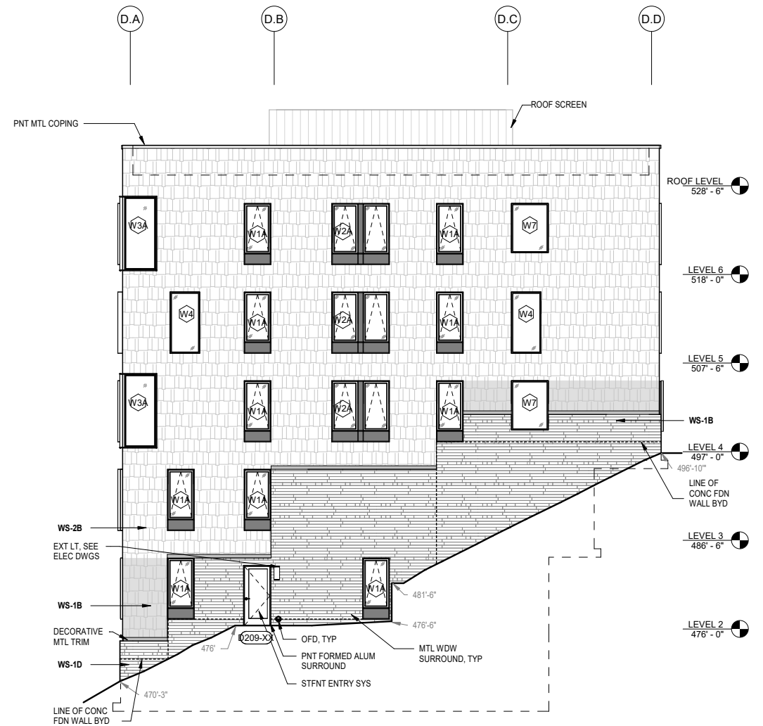
2 EXTERIOR ELEVATION - WING D - WEST A313 1/16" = 1'-0"
