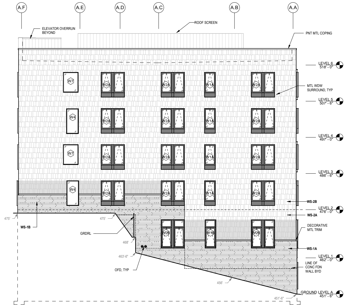
2 EXTERIOR ELEVATION - WING A - EAST A310 1/16" = 1'-0"
