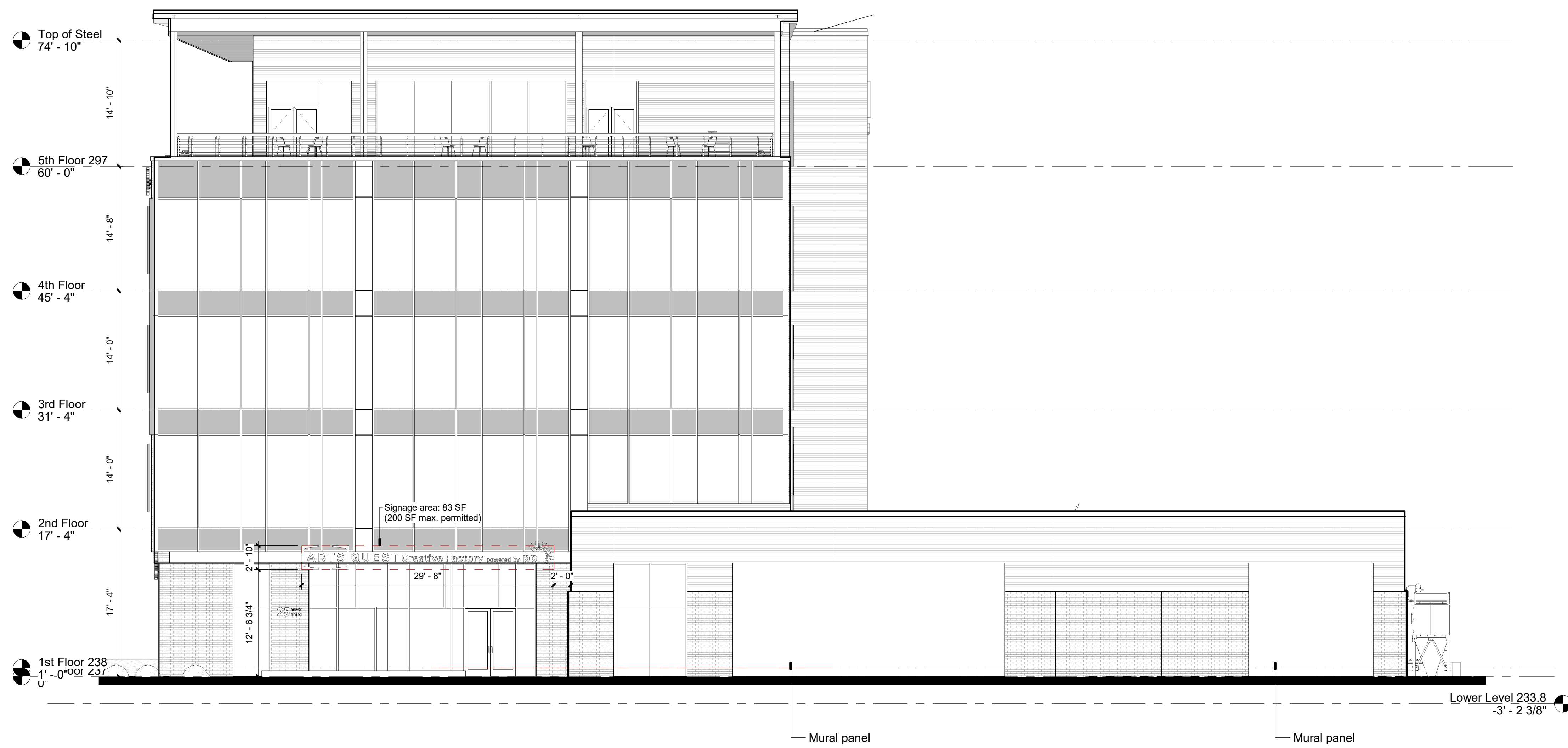
2 East Elevation - HCC Signage 1/8" = 1'-0"
