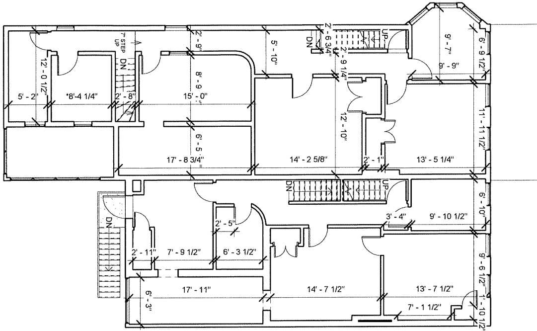
① 230-232 Second Floor 11x17 1/8" = 1'-0"
