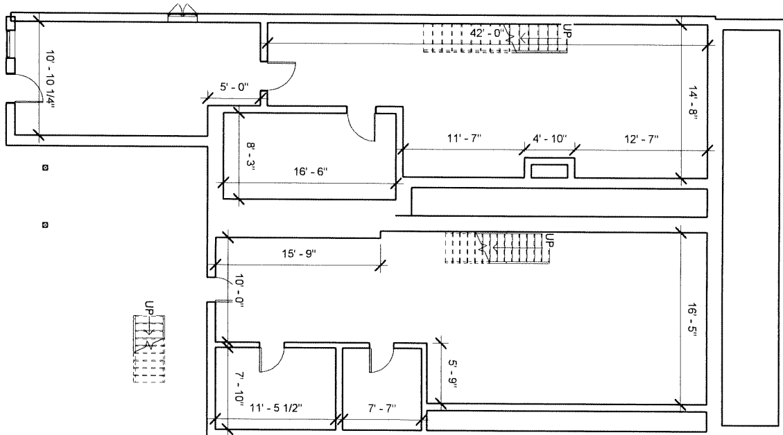
1 230-232-Basement 11x17 1/8" = 1'-0"
