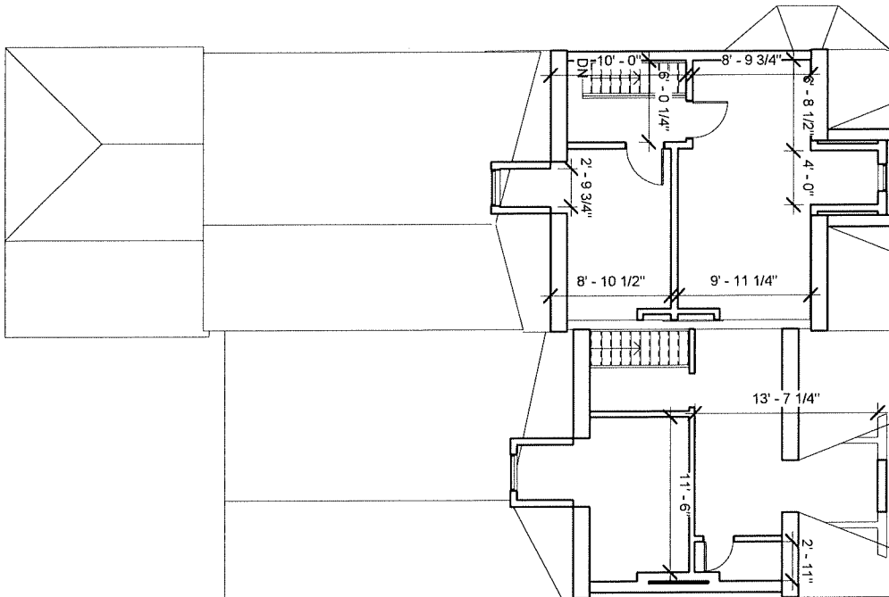
② 230-232 THIRD FLOOR 1/8" = 1'-0"
