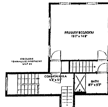
Unit 4 3rd floor
