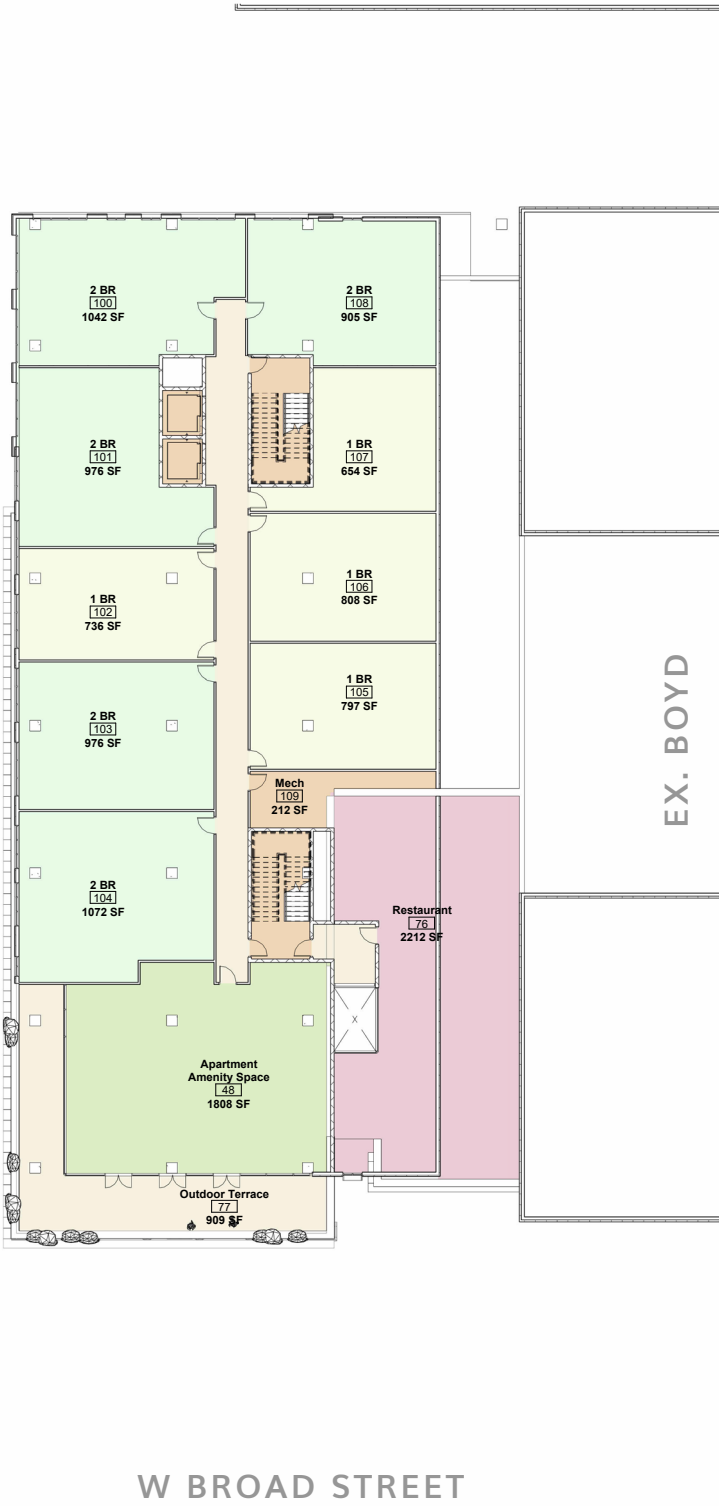
AMENITIES FLOOR (03)
