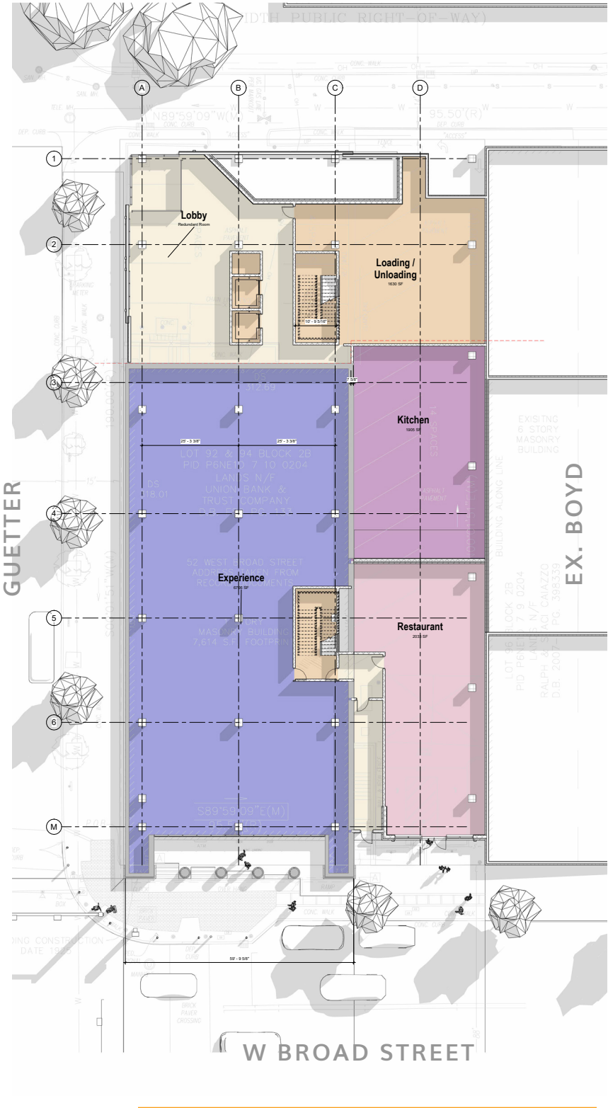
GROUND LEVEL (01)
