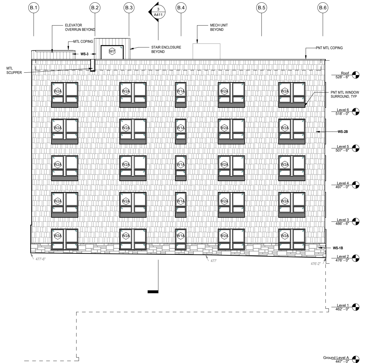
3 A311 EXTERIOR ELEVATION - WING B - SOUTH 1/16" = 1'-0"
