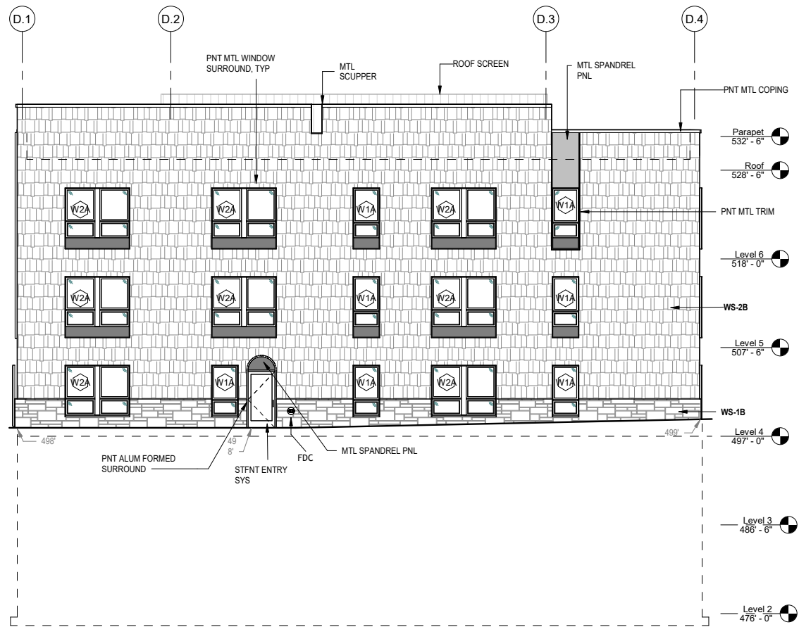
3 EXTERIOR ELEVATION - WING D - SOUTH A313 1/16" = 1'-0"
