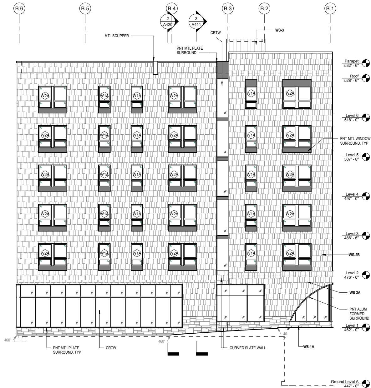
1 A311 EXTERIOR ELEVATION - WING B - NORTH 1/16" = 1'-0"
