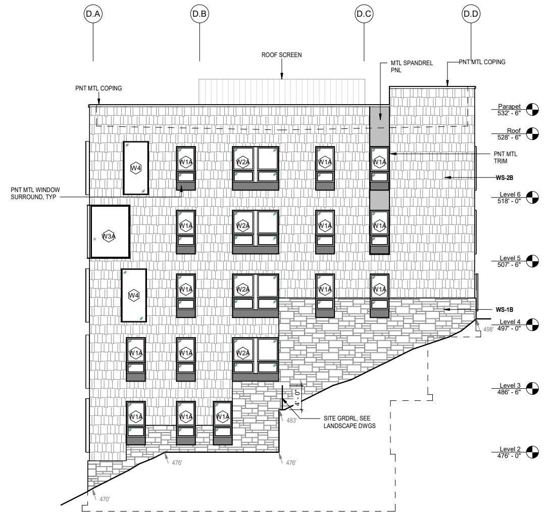
4 EXTERIOR ELEVATION - WING D - WEST A313 1/16" = 1'-0"
