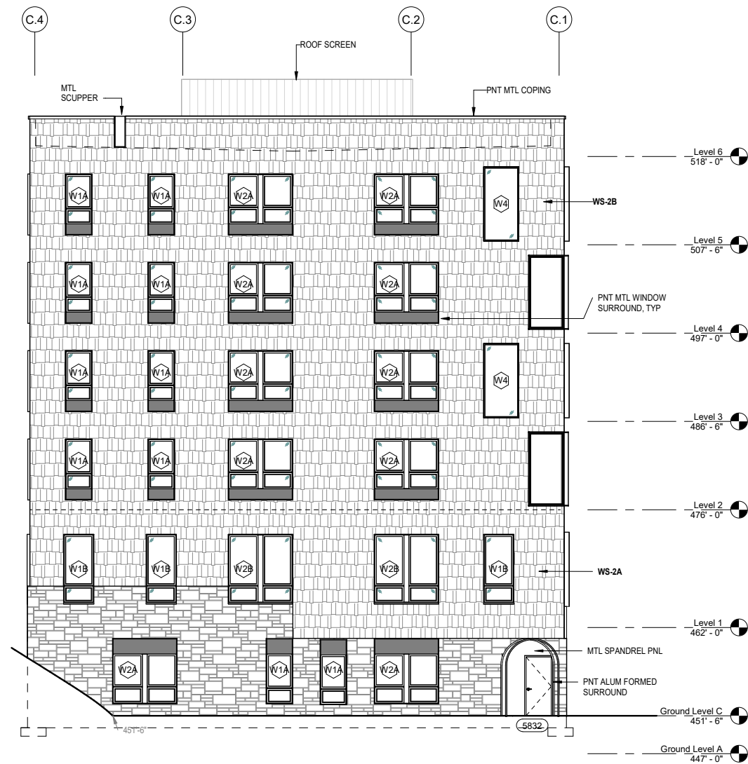
1 EXTERIOR ELEVATION - WING C - NORTH A312 1/16" = 1'-0"
