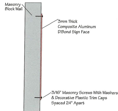
Side View Dibond Sign Mounting to Wall
