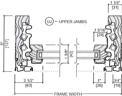
REPLACE EXISTING PELLA LIFESTYLE SERIES ALUMINUM CLAD WOOD COLOR: BRICK RED SEE JAMB BELOW
