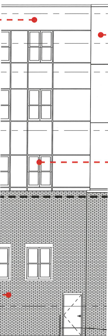
AT ADDITION & EXISTING PAINTED BRICK PELLA LIFESTYLE SERIES ALUMINUM CLAD WOOD COLOR: FOSSIL SEE HEAD, SILL, AND CHECK RAIL BELOW
