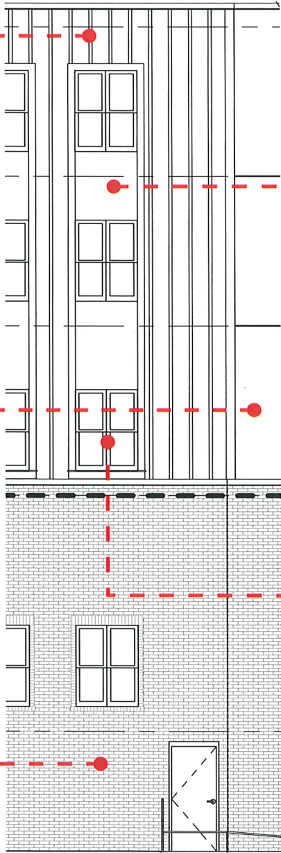
WEST ELEVATION
