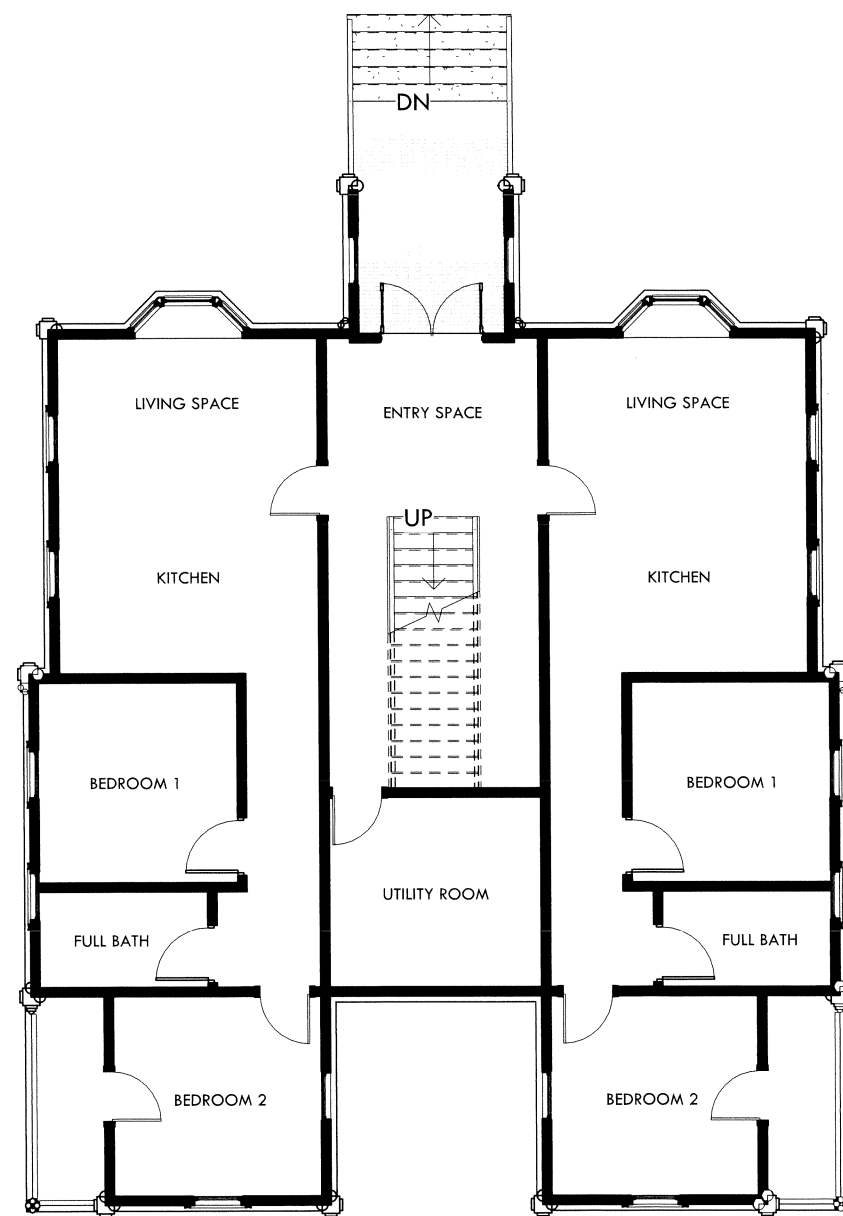
LEVEL 1 FLOOR PLAN
