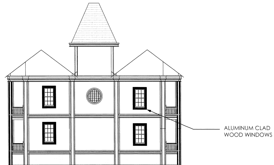
SOUTH ELEVATION
