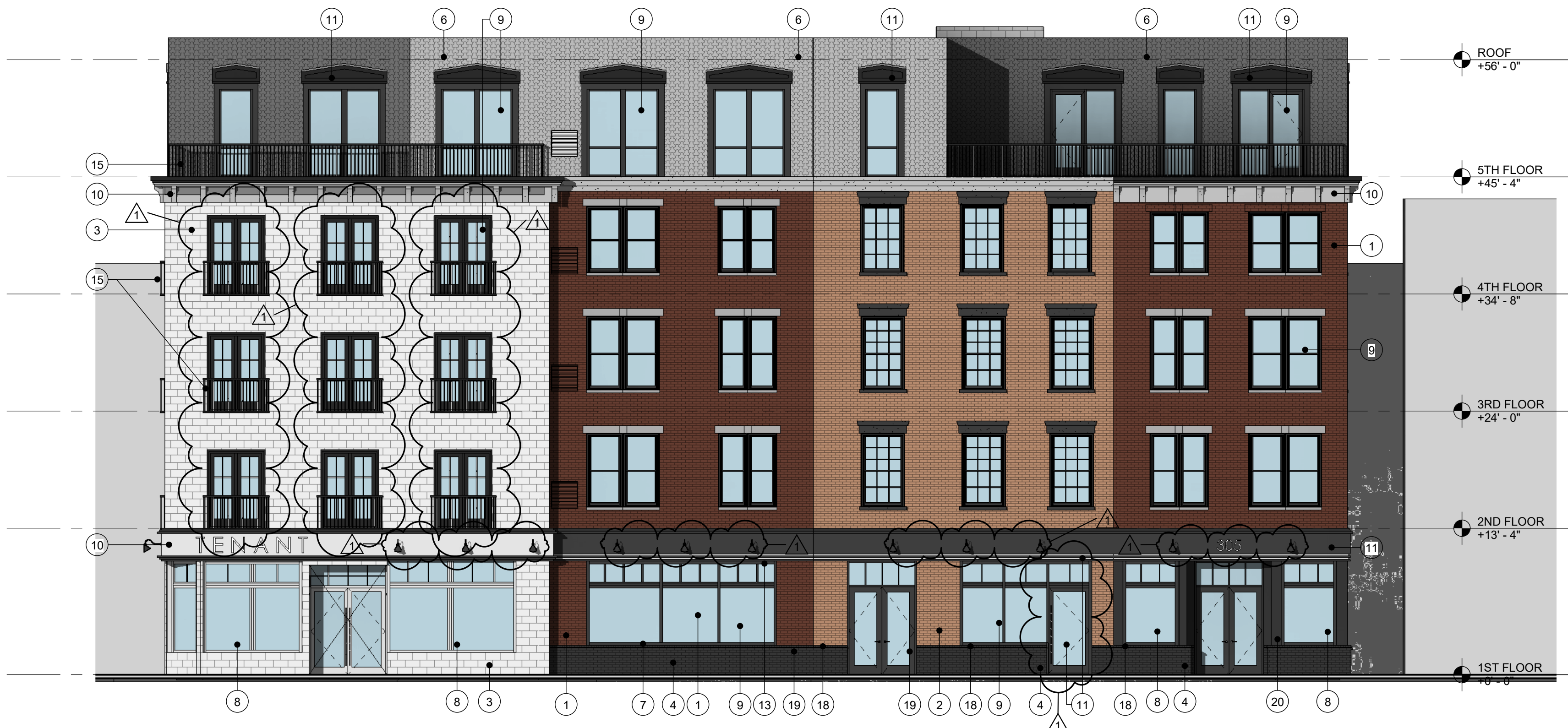
(C) SOUTH ELEVATION - E 3RD ST SCALE: 1/8" = 1'-0"
