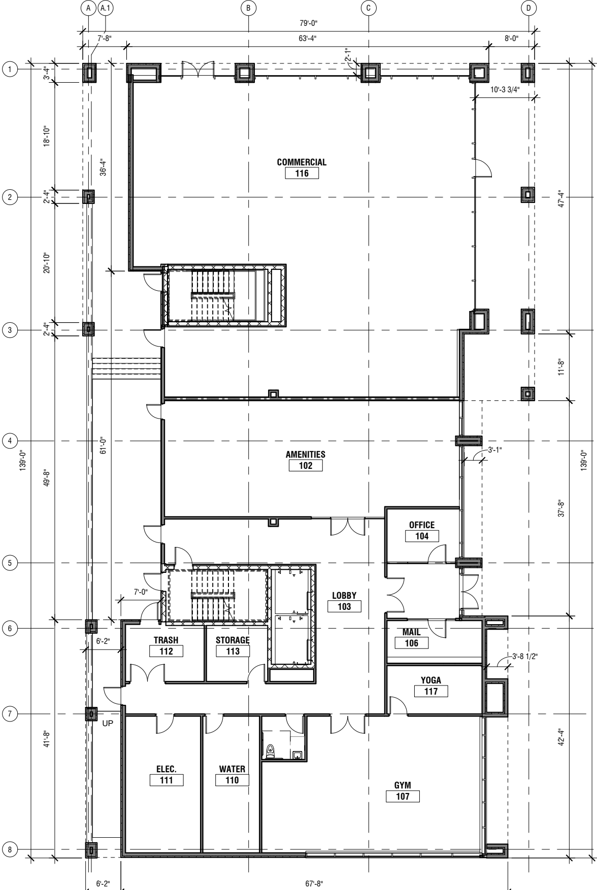
FIRST FLOOR
