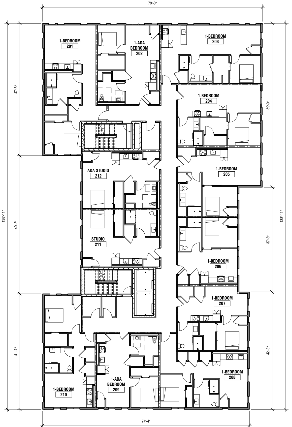
SECOND FLOOR
