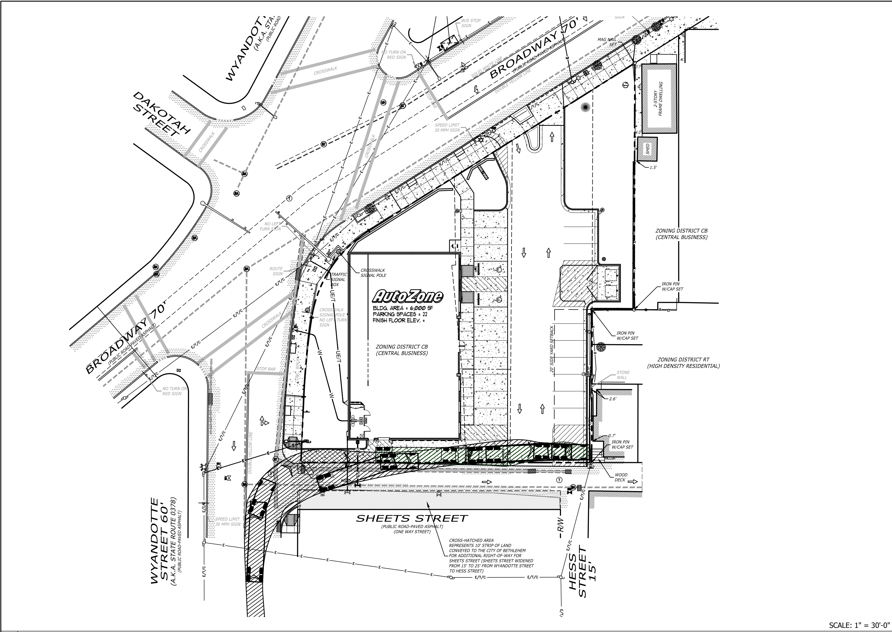
1 WB-50 TRUCK ENTRY- WYANDOTTE STREET TO SHEETS STREET
