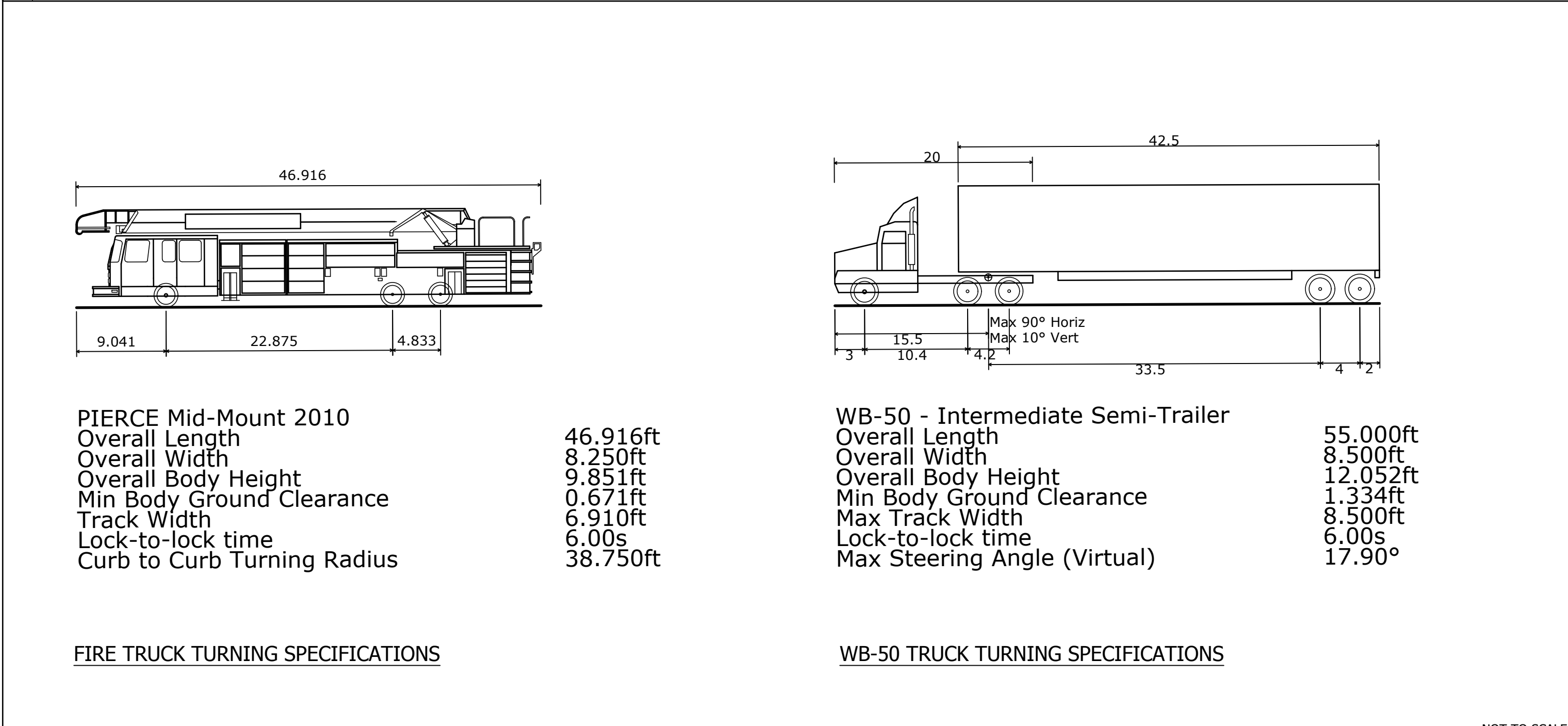
4 TRUCK TURNING PROFILES
