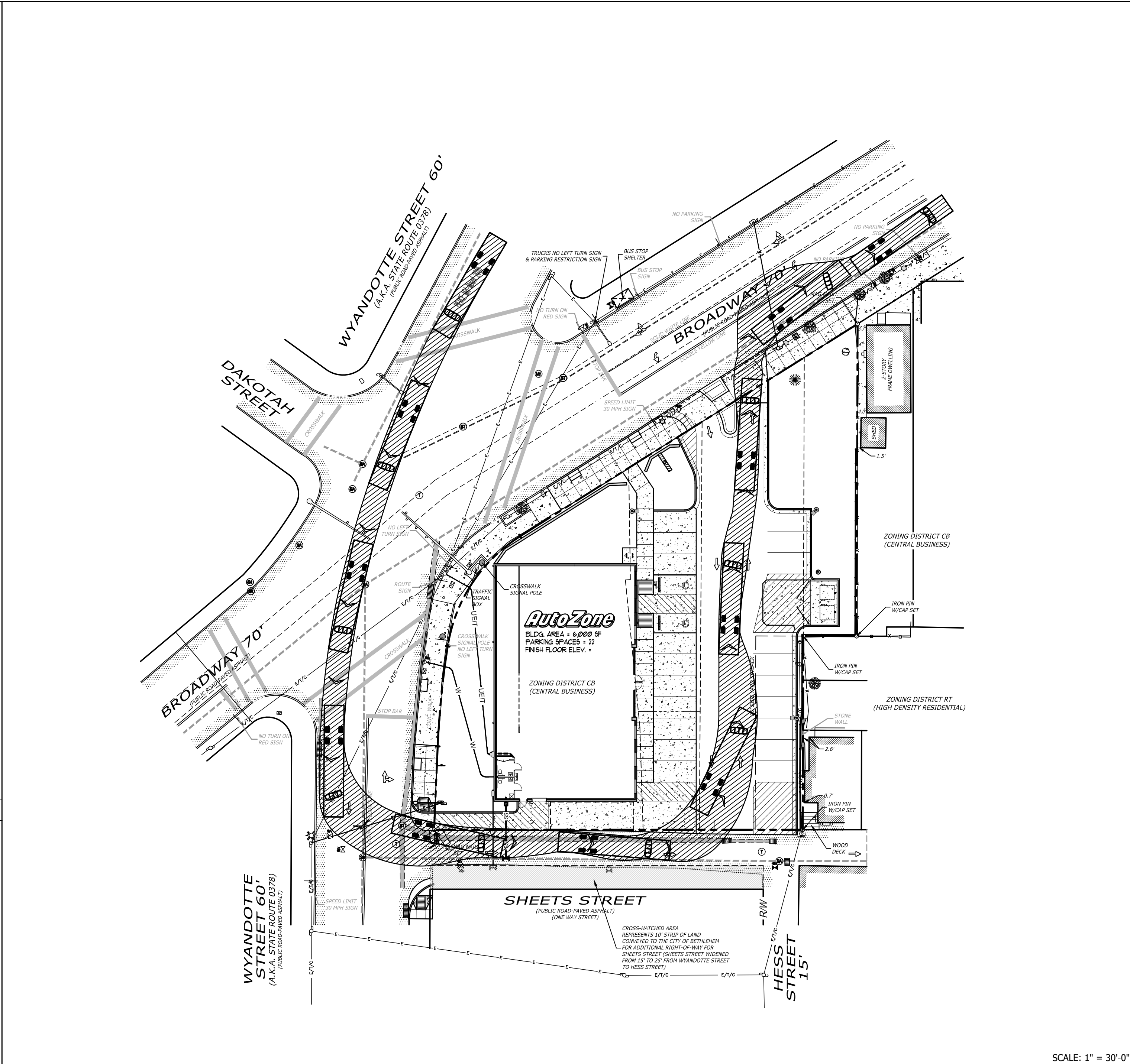
3 FIRE TRUCK ENTER & EXIT
