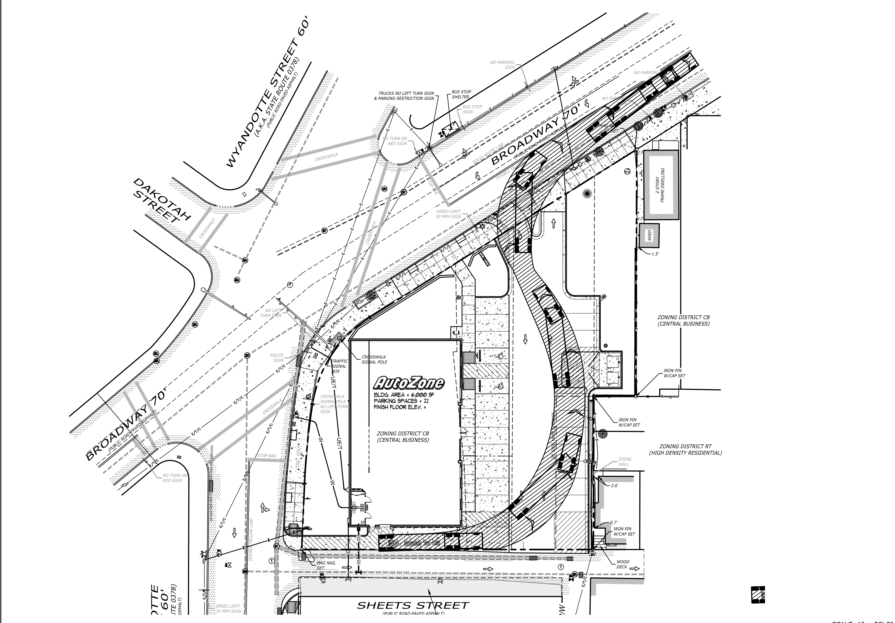
2 WB-50 TRUCK EXIT - BROADWAY (EASTBOUND)
